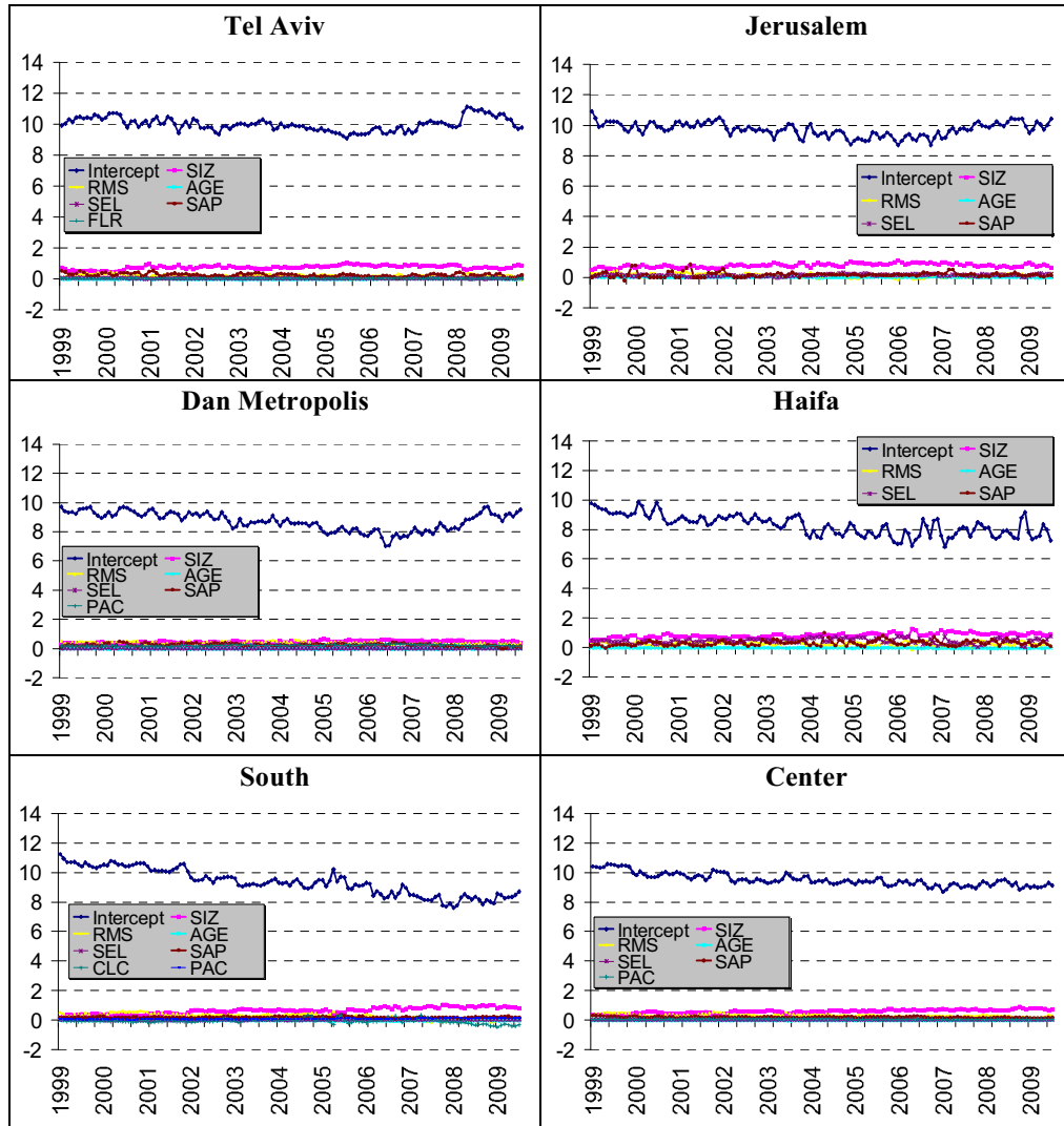
Graph 15 Change in Coefficients over Time
