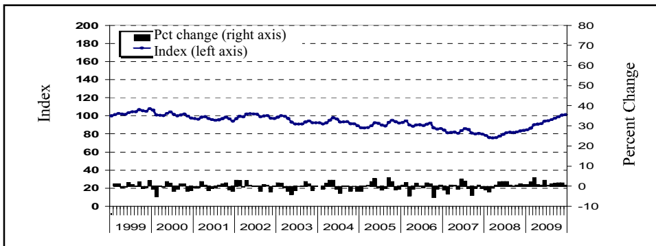
Graph 5 Behavior of Haifa Index
