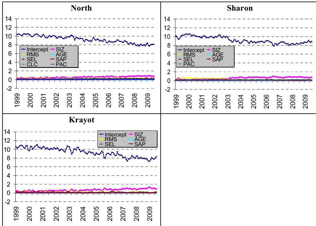
Graph 15 Change in Coefficients over Time
