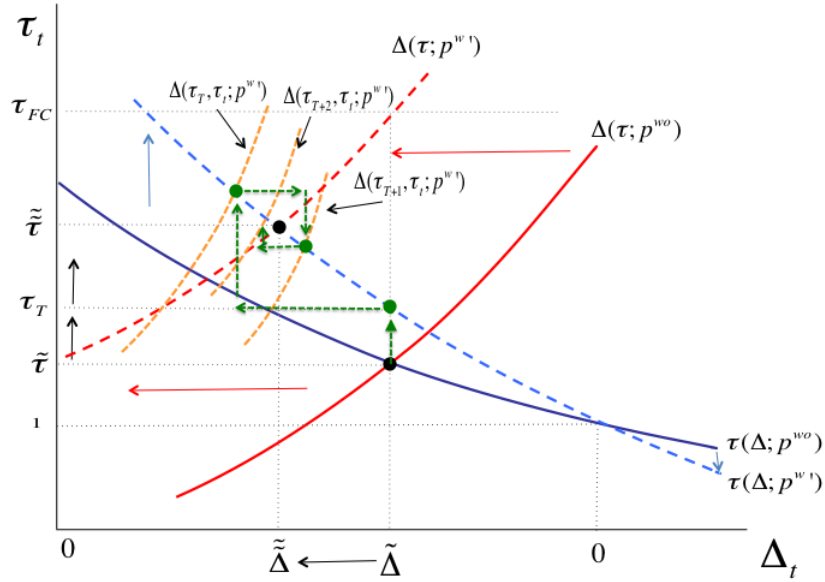
Figure A.2: Escalation in (\Delta, \tau)
