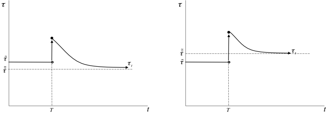
Figure 5: Protectionist Overshooting: Dynamic Tariff Response to p^w \uparrow if \Delta'(p) > 0 .
