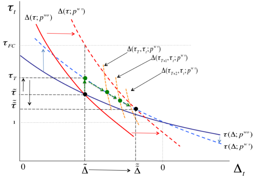
Figure A.1: Overshooting (\Delta, \tau)
