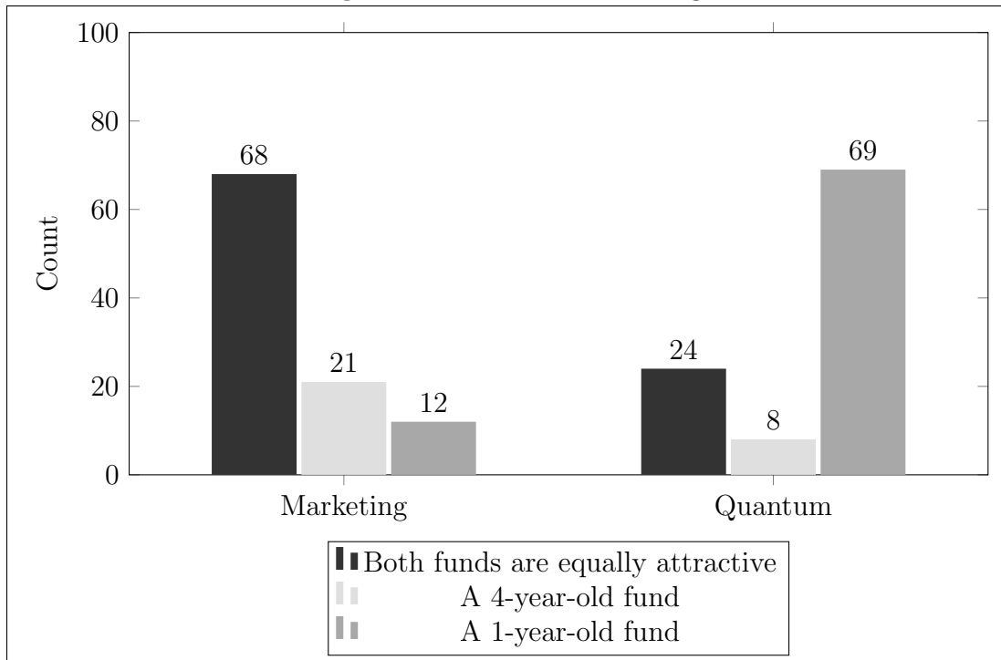
Figure 5. Scenario 1: Fund Age
