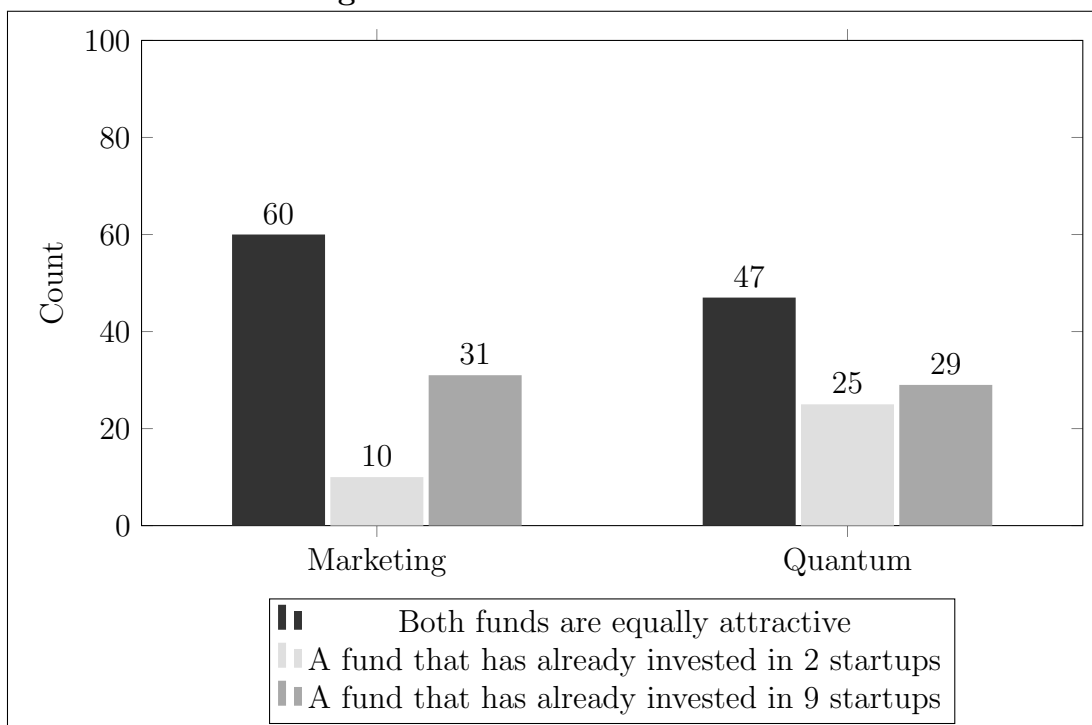
Figure 10. Scenario 6: Portfolio Size
